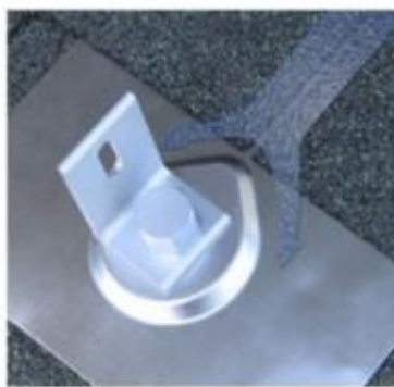
Flashing designed to redirect water flow.
